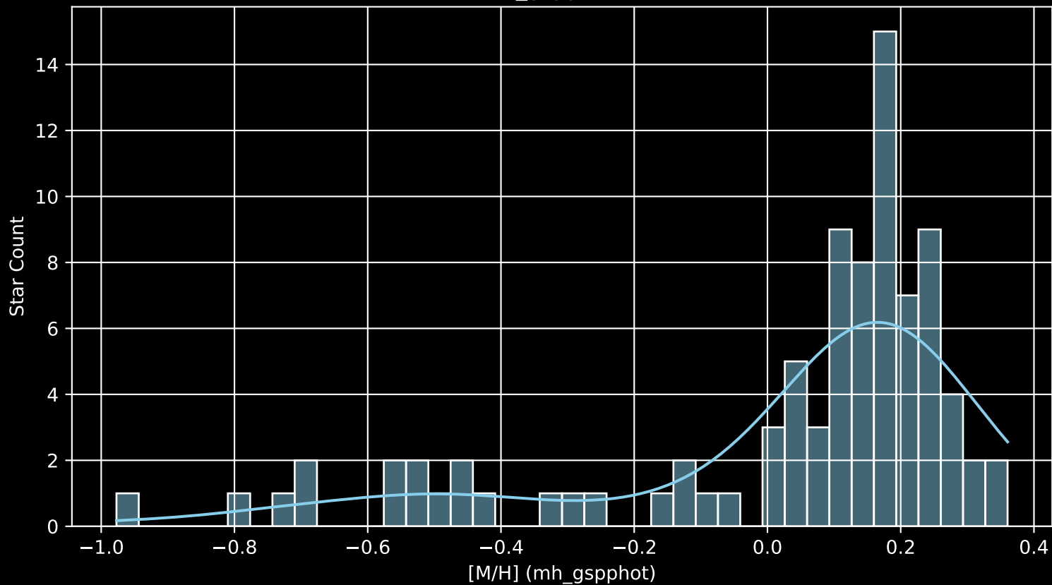
APOGEE DR17 Field: [LMC22 [M/H] (mh_gspphot) (n= 88)
