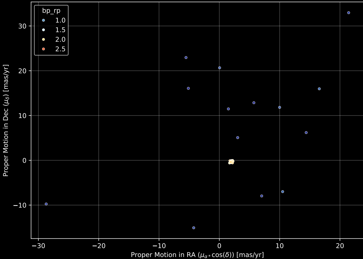
APOGEE DR17 Field: [LMC22] Proper Motion Diagram (n= 88)
