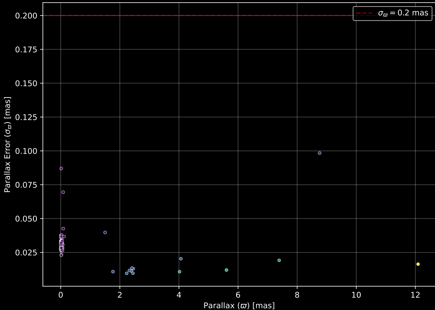
APOGEE DR17 Field: [LMC22] Parallax Quality (n= 88)
