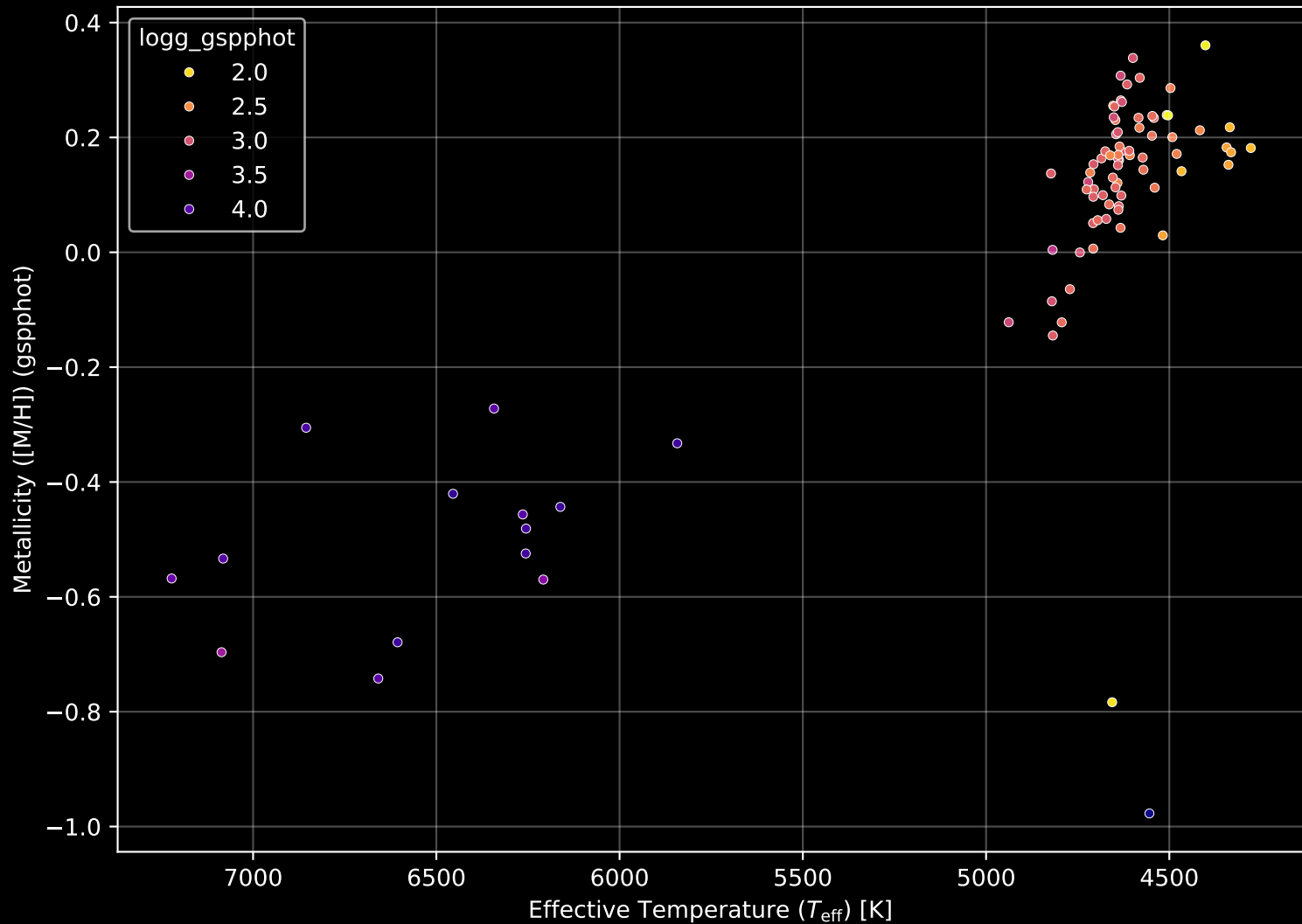
APOGEE DR17 Field: [LMC22] Stellar Population Parameters (n= 88)
