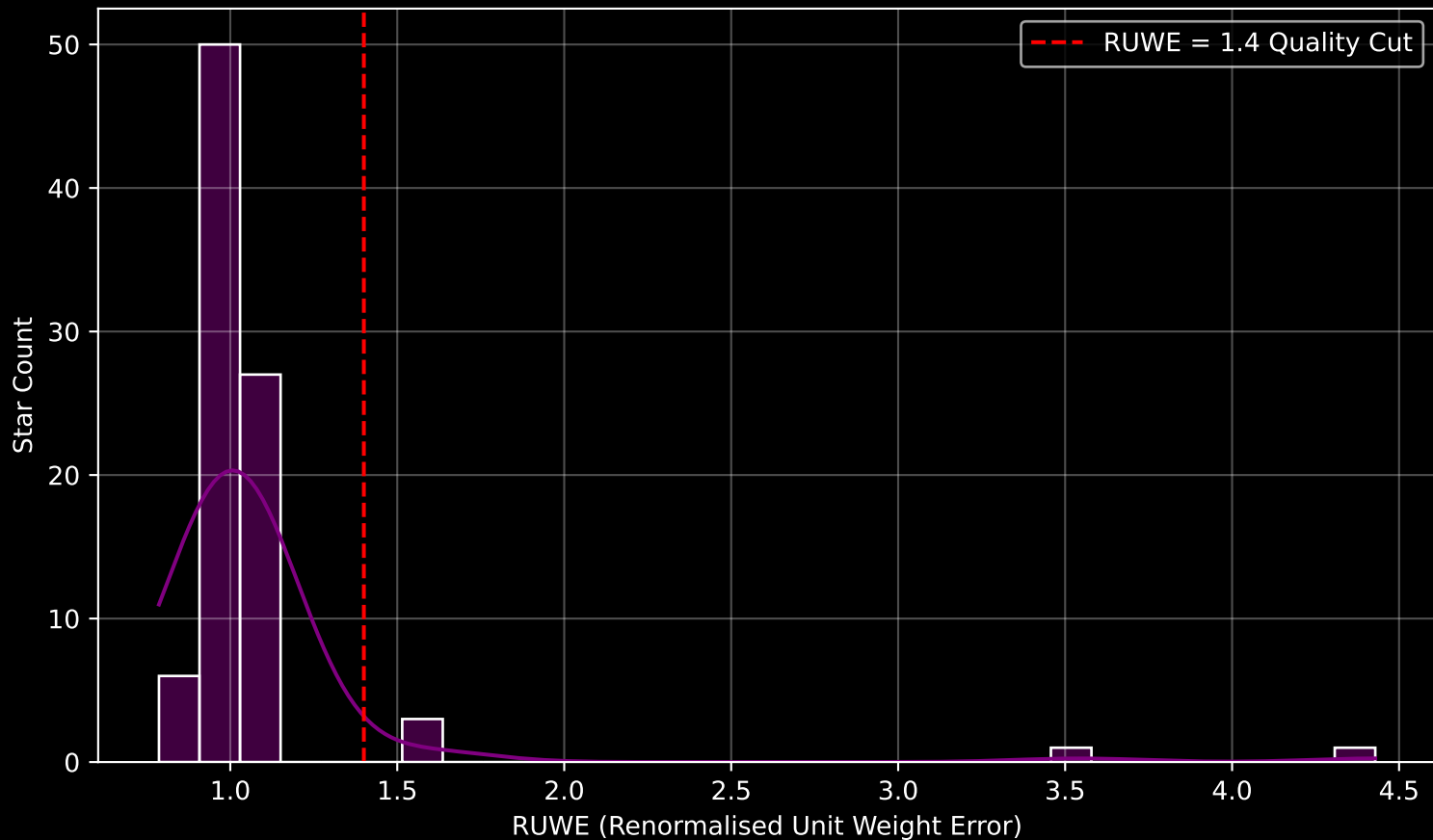
GAPOGEE DR17 Field [LMC22] RUWE Distribution (n= 88)
